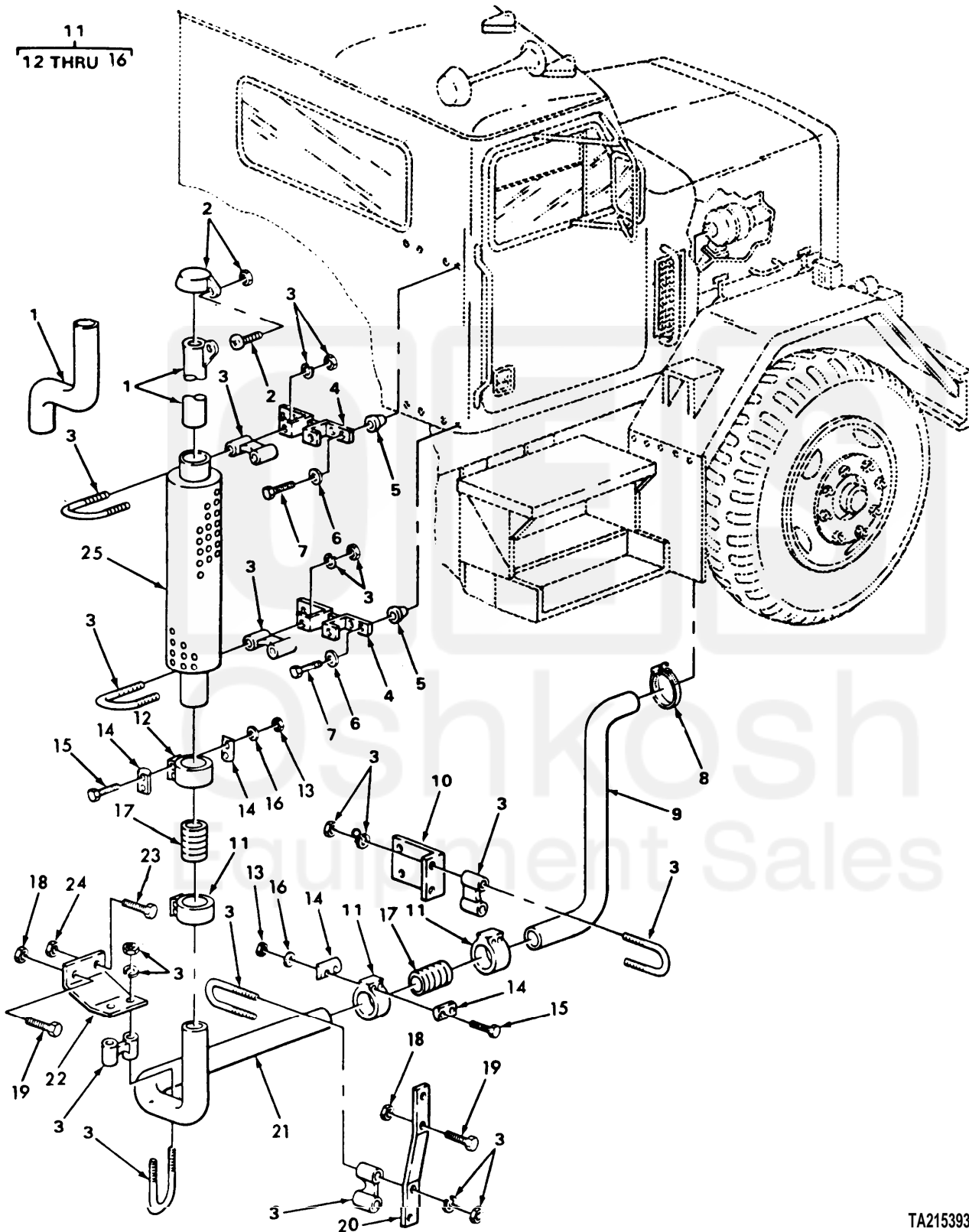
FIGURE 18. EXHAUST SYSTEM.
